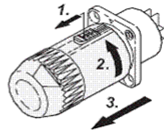
To disengage, pull back lock, rotate anti-clockwise and part.
